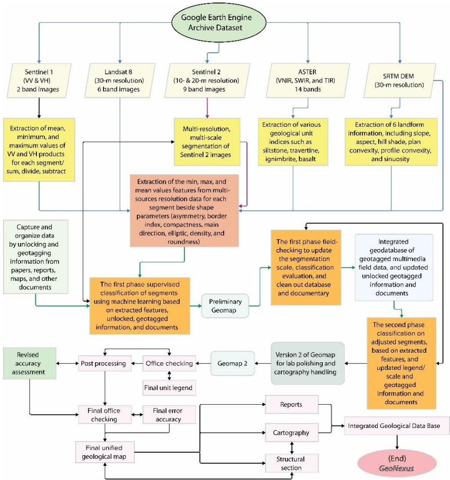
Figure 21: Flowchart of the upgraded logical tree for the preparation of base server thematic maps based on the use of the processing platform
